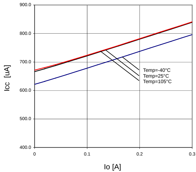
Figure 30. I_o - I_{CC}
