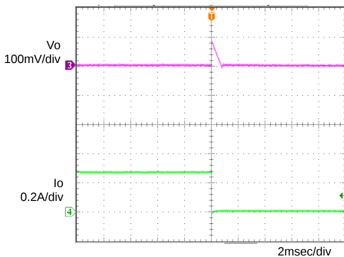
Figure 6. Transient Response (0.3→0A) Co=1\mu F , T_a=-40^\circ C
