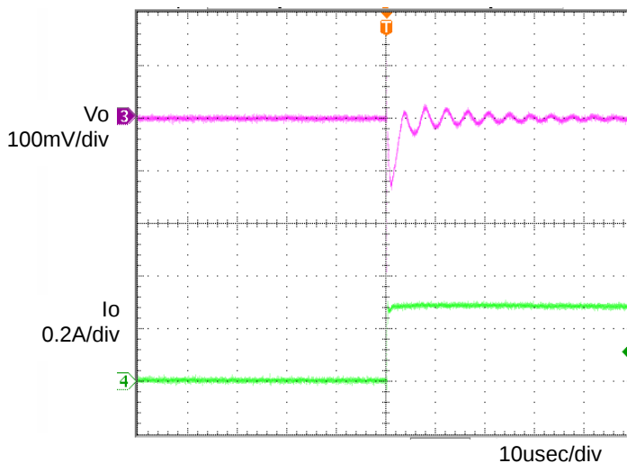
Figure 4. Transient Response (0→0.3A) Co=1\mu F , T_a=25^\circ C
