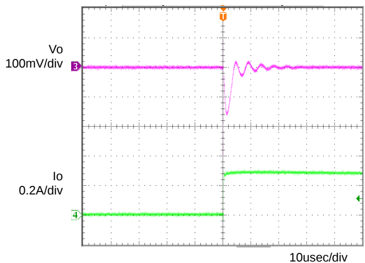
Figure 5. Transient Response (0→0.3A) Co=1\mu F , T_a=105^\circ C
