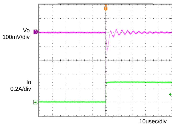
Figure 3. Transient Response (0→0.3A) Co=1\mu F , T_a=-40^\circ C
