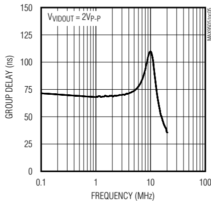
GROUP DELAY
