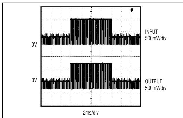
Figure 4. DirectDrive Output
