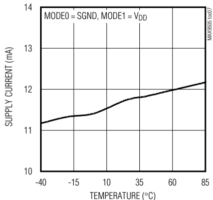
QUIESCENT SUPPLY CURRENT vs. TEMPERATURE (VIDEO MODE)
