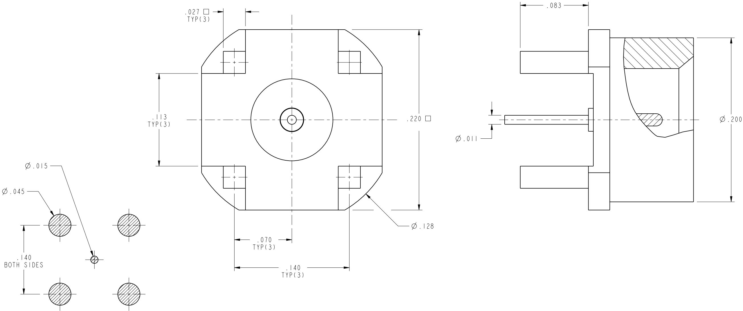
RECOMENDED PCB MOUNTING DIMENSIONS
