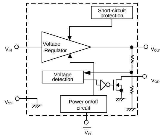
Figure 2 Block Diagram
