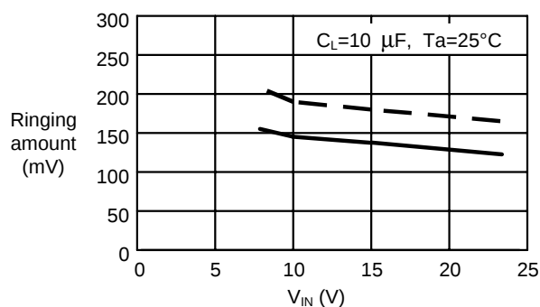
3. V_{IN} Dependency
