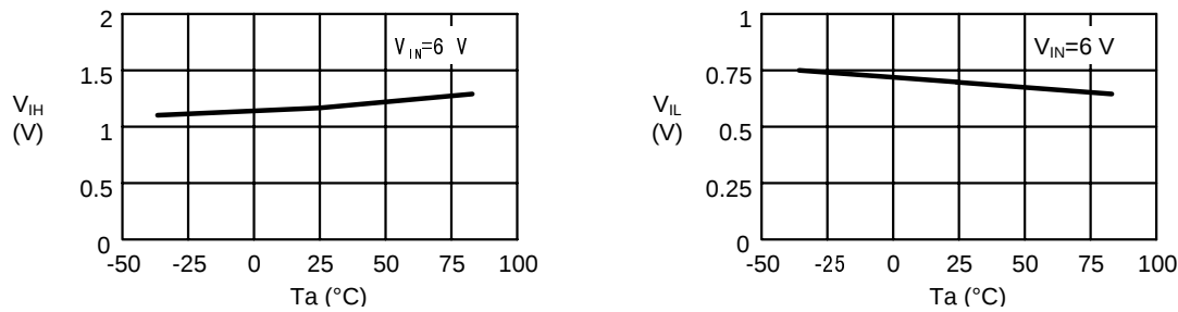
(a) High Level Input Voltage ( V_{IH} ) - Temperature ( T_a ) (b) Low Level Input Voltage ( V_{IL} ) - Temperature ( T_a )
