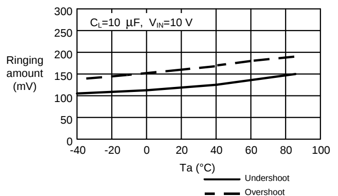
4. Temperature Dependency
