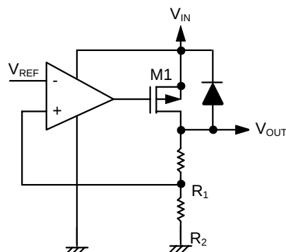
Figure 7 Voltage Regulator
