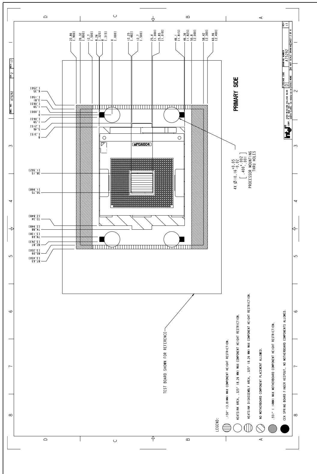
Figure 3-5. Top Side Board Keepout Zones (Part 2)
