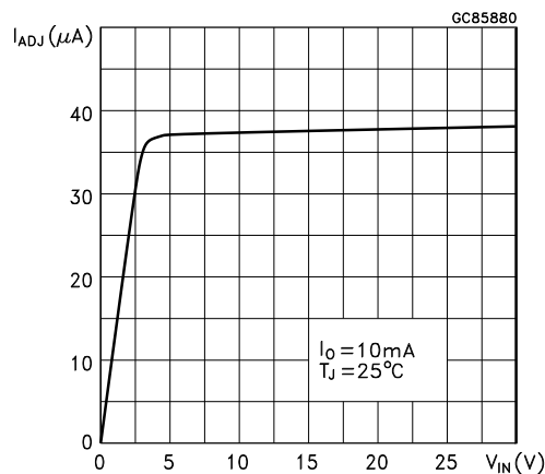
Figure 11. Adjust pin current vs. input voltage
