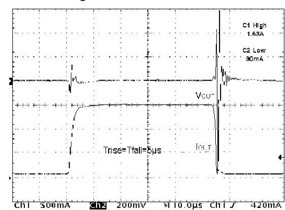
Figure 25. Load transient
