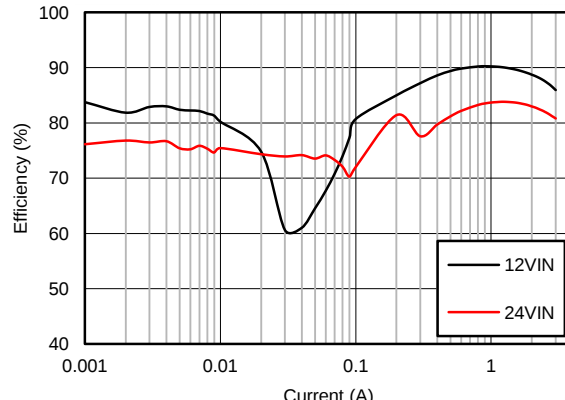
Figure 80. Efficiency
