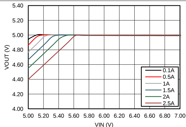
Figure 82. Dropout Curve
