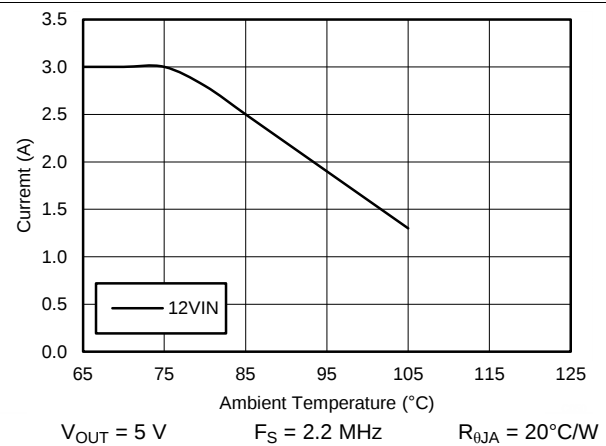
Figure 90. Derating Curve
