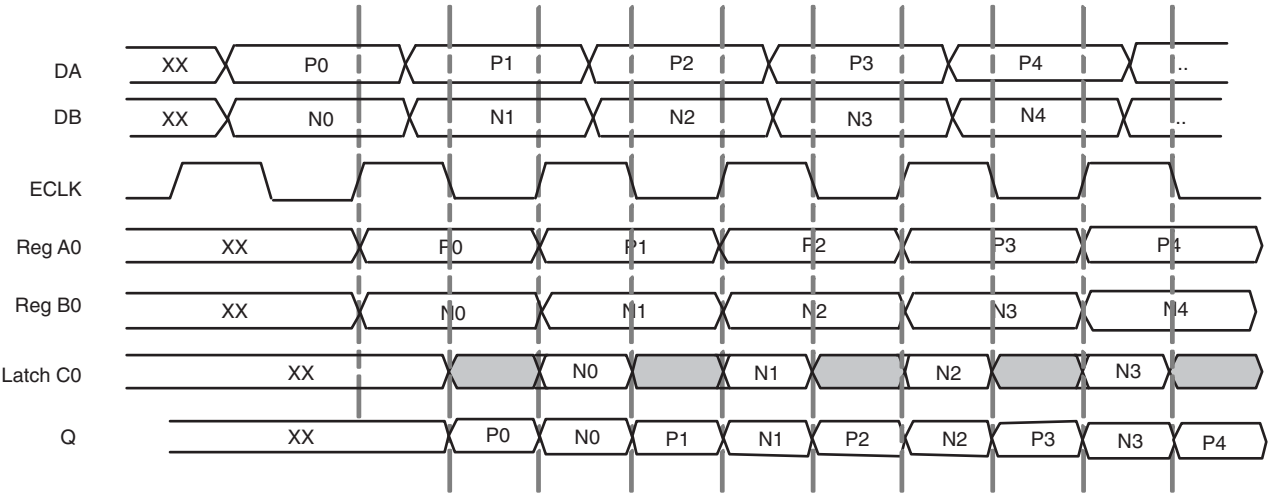
Figure 12-37. ODDRXC Waveform
