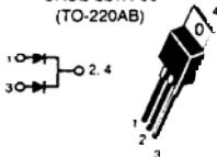
Case 221A-06 (TO-220AB)
