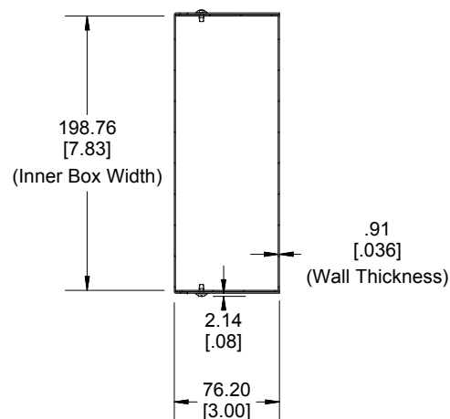
SECTION A-A End View of Assembly
