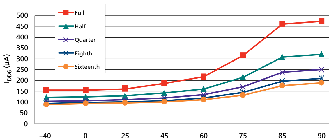
Figure 7: Typical Self Refresh Current vs. Temperature
