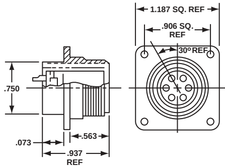
7-8905 97-3102A14S-6S (639) with insert rotated 30° off normal position between contacts "A" and "F".
