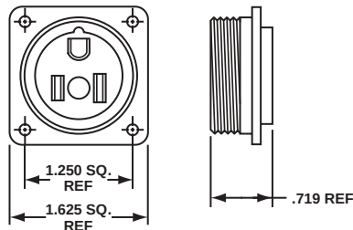
7-8648-5 Convenience outlet with metal cap and chain
