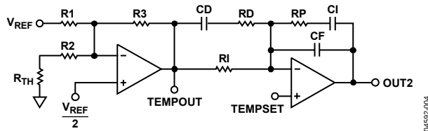
Figure 3. Temperature and Compensation Network Circuits
