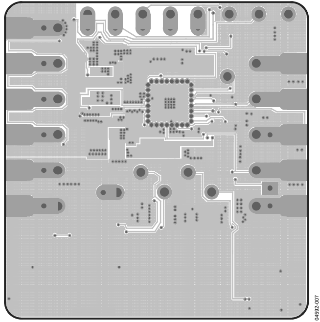
Figure 12. Bottom Layer Layout (Mirrored)
