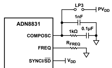
Figure 7. Switching Frequencies
