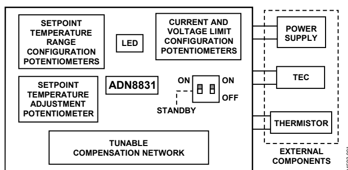
Figure 1. Functional Block Diagram of ADN8831 Evaluation Board
