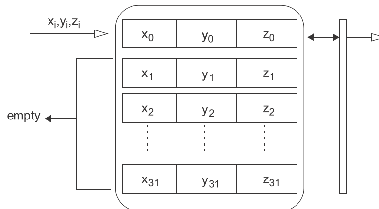
Figure 7. Bypass mode
