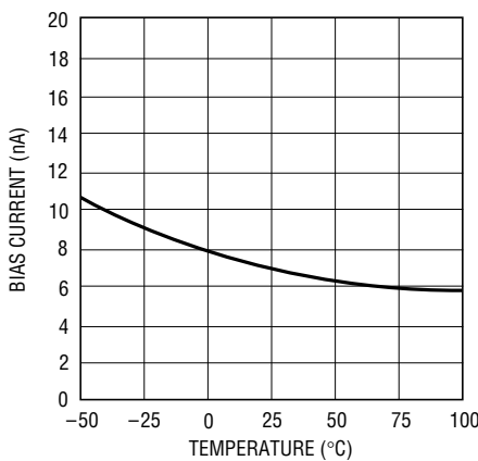
LB1 Pin Bias Current
