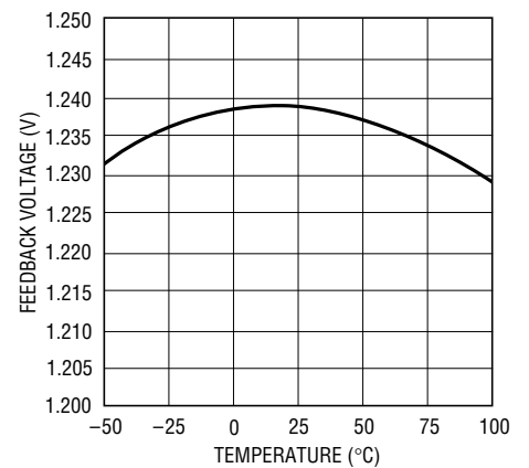
FB Voltage
