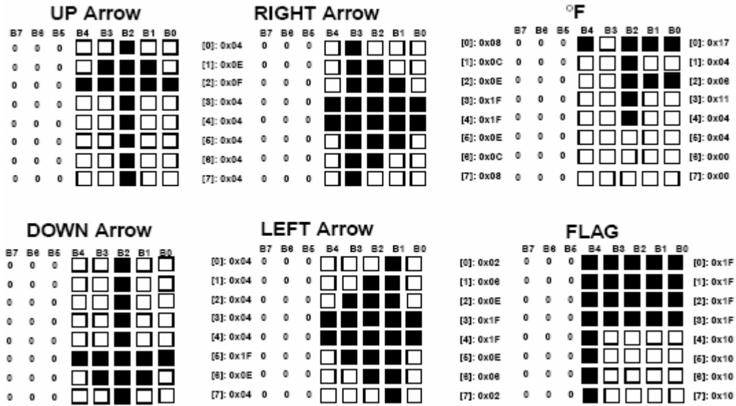
Figure 3-3, Examples of custom symbols
