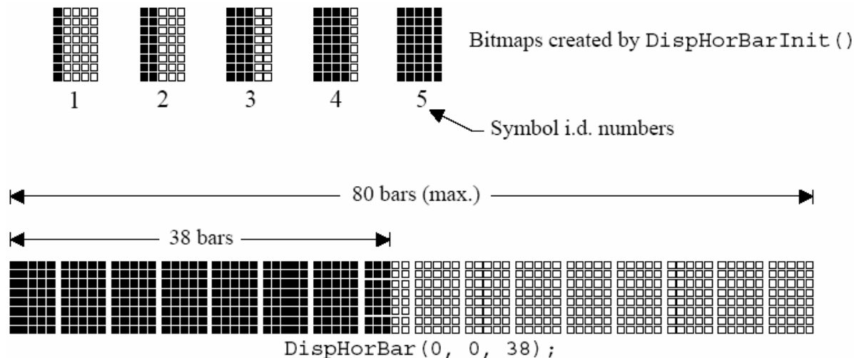
Figure 3-4, Bargraphs with 16-character displays
