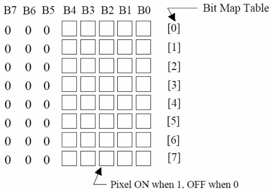
Figure 3-2, Defining custom characters
