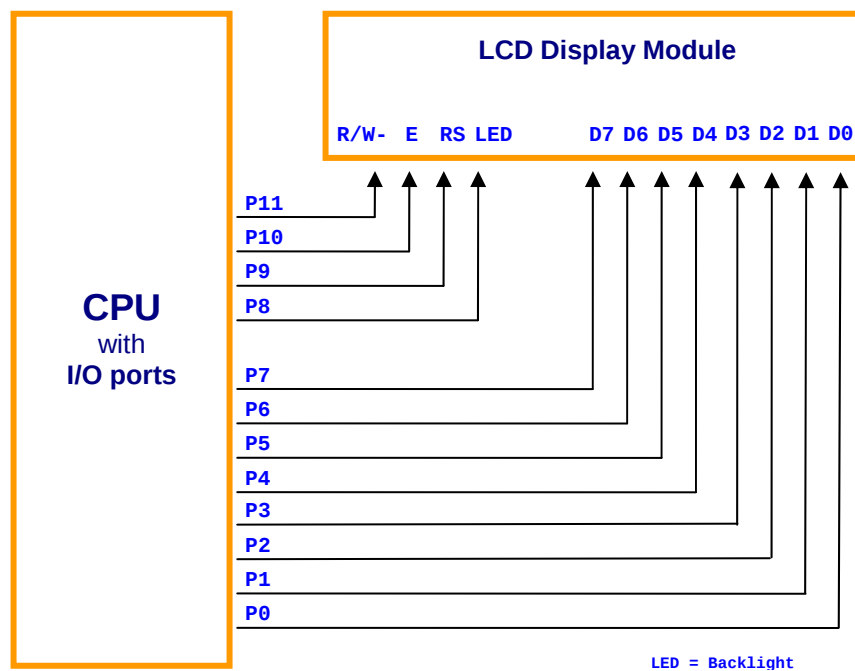
Figure 1-2, Interfacing to an HD44780-based LCD module (8-bit interface)
