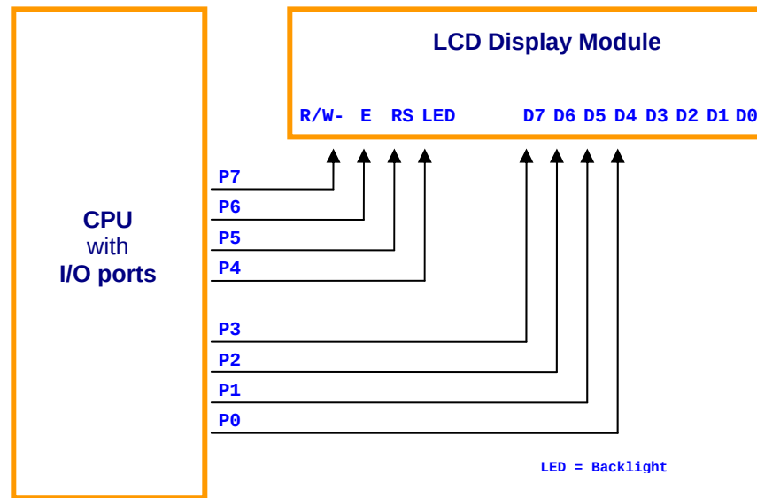
Figure 1-1, Interfacing to an HD44780-based LCD module (4-bit interface)
