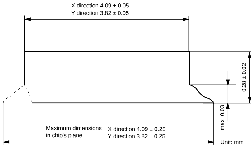
Figure F.3 Cross-Sectional View of Chip (HCD64F38004 and HCD64F38002)
