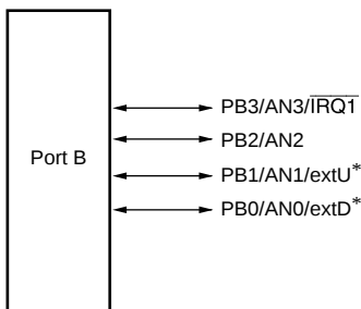
Figure 8.10 Port B Pin Configuration
