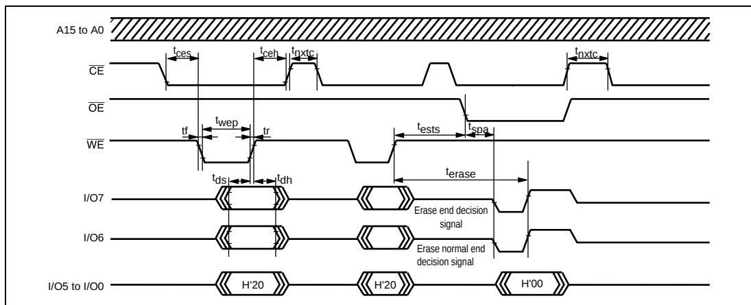
Figure 6.18 Timing Waveforms in Auto-Erase Mode
