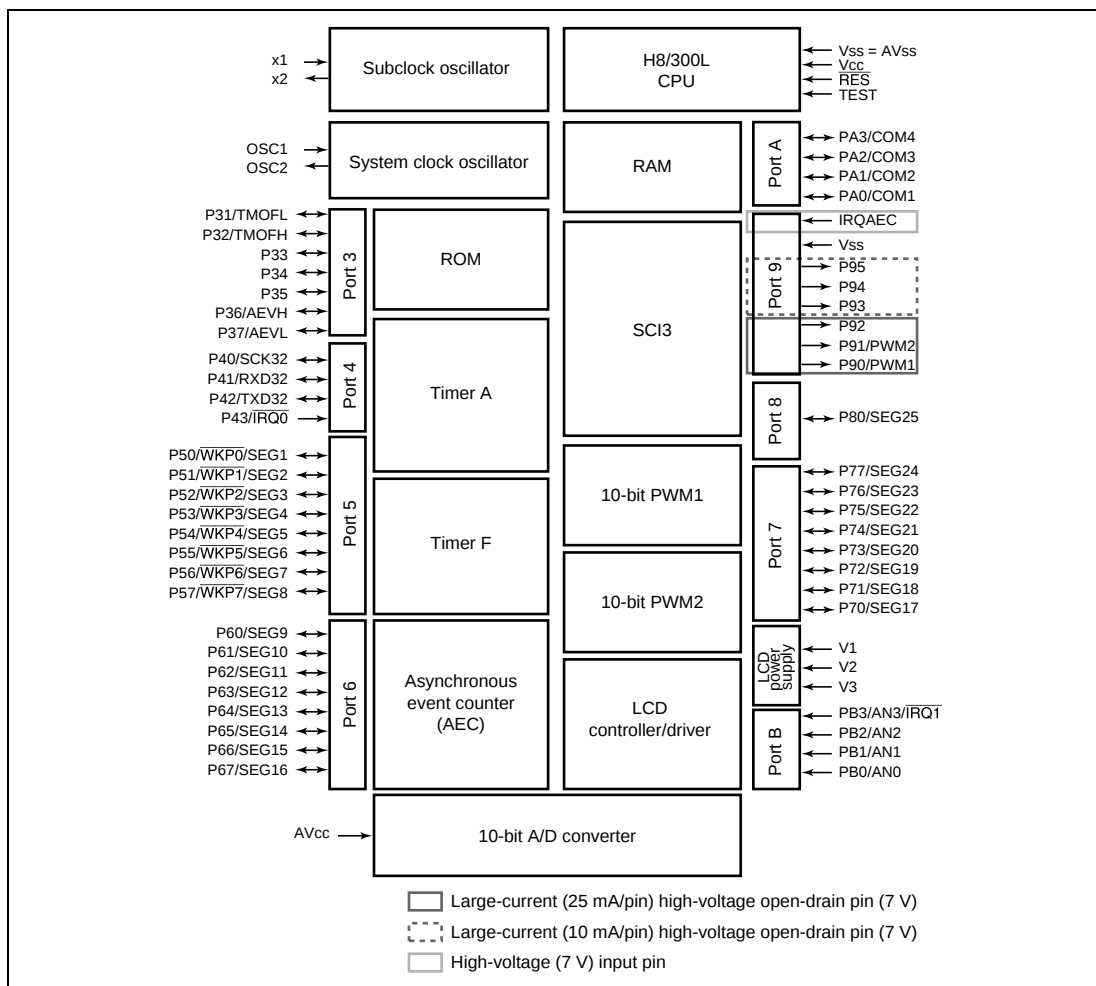
Figure 1.1 Internal Block Diagram of H8/3802 Group
