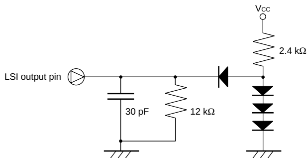
Figure 17.6 Output Load Circuit
