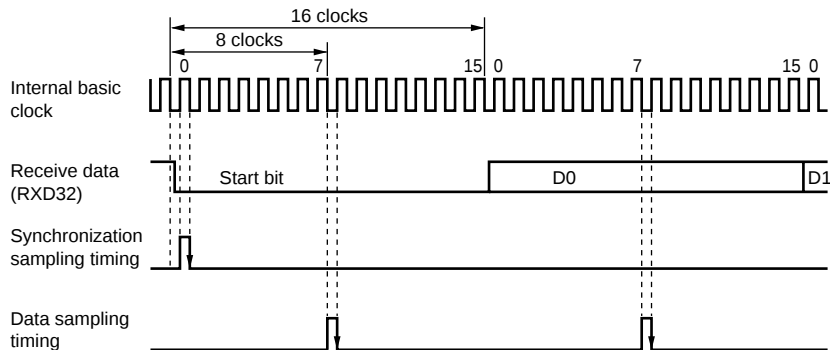
Figure 10.20 Receive Data Sampling Timing in Asynchronous Mode
