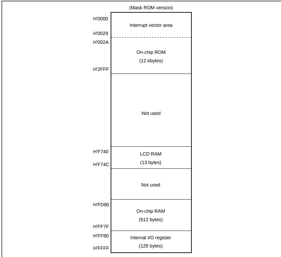
Figure 2.1(7) H8/38001, H8/38101 Memory Map
