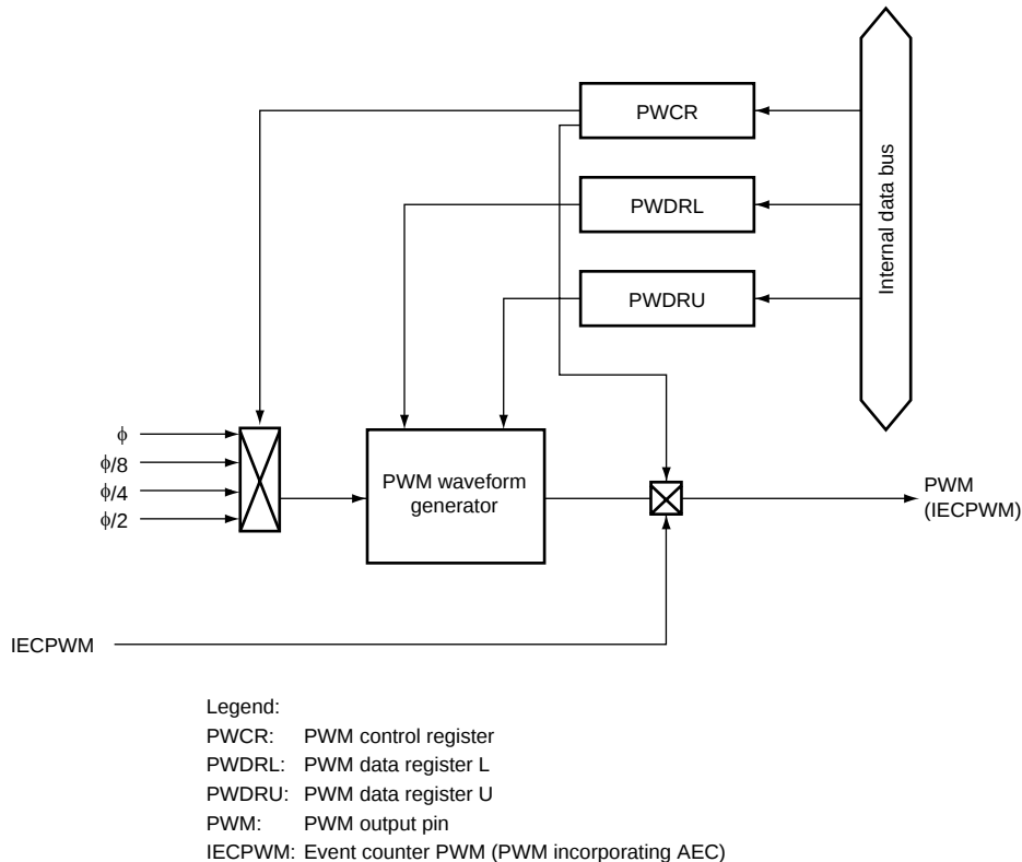
Figure 11.1(2) Block Diagram of 10-Bit PWM (H8/38104 Group)
