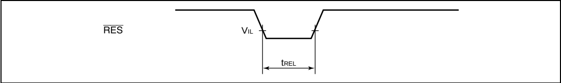
Figure 17.2 \overline{RES} Low Width Timing
