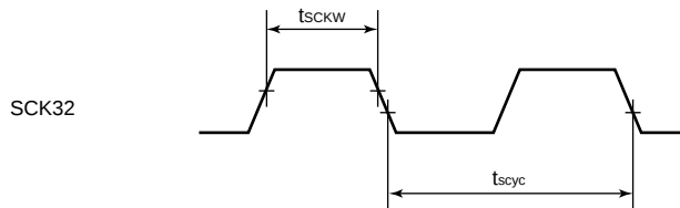
Figure 17.4 SCK3 Input Clock Timing
