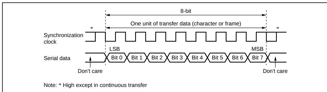
Figure 10.9 Data Format in Clocked Synchronous Communication
