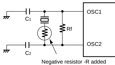
Negative resistor -R added (1) Negative resistor measurement circuit
