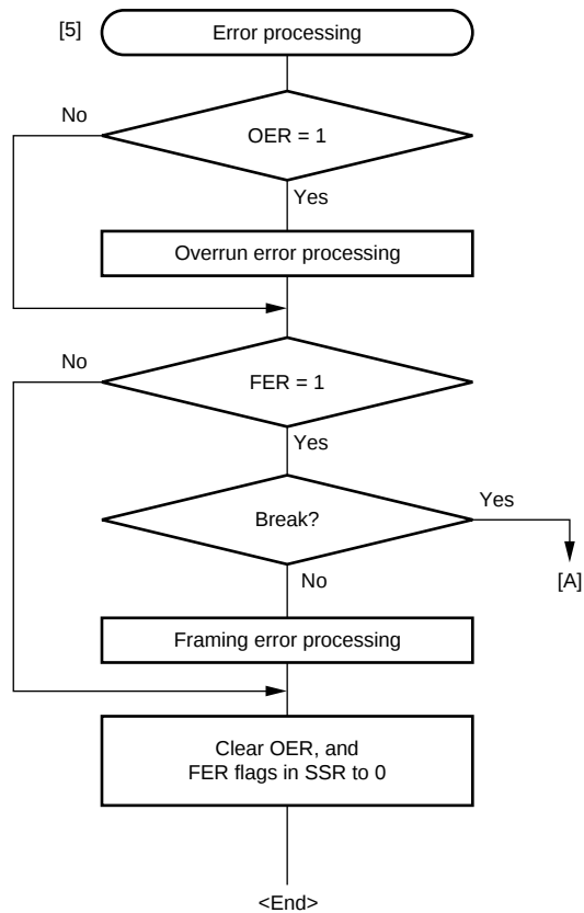
Figure 10.17 Sample Multiprocessor Serial Reception Flowchart (2)
