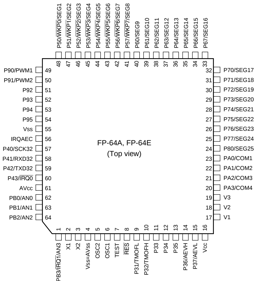
Figure 1.4 Pin Arrangement of H8/3802 and H8/38004 Group (FP-64A, FP-64E)
