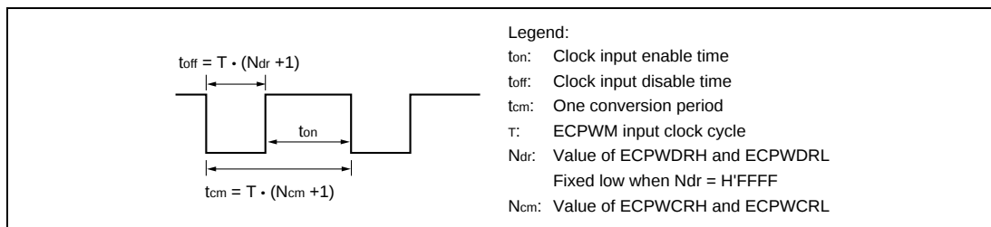
Figure 9.10 Event Counter Operation Waveform
