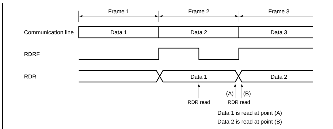
Figure 10.21 Relation between RDR Read Timing and Data
