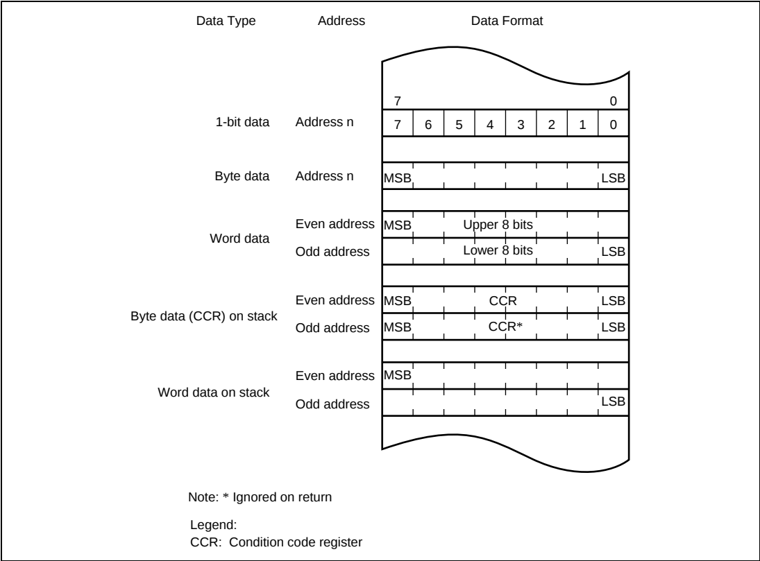
Figure 2.5 Memory Data Formats
