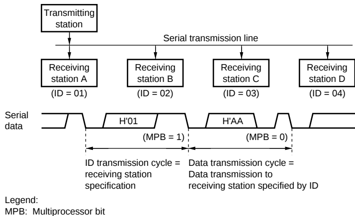
Figure 10.15 Example of Communication Using Multiprocessor Format (Transmission of Data H'AA to Receiving Station A)
