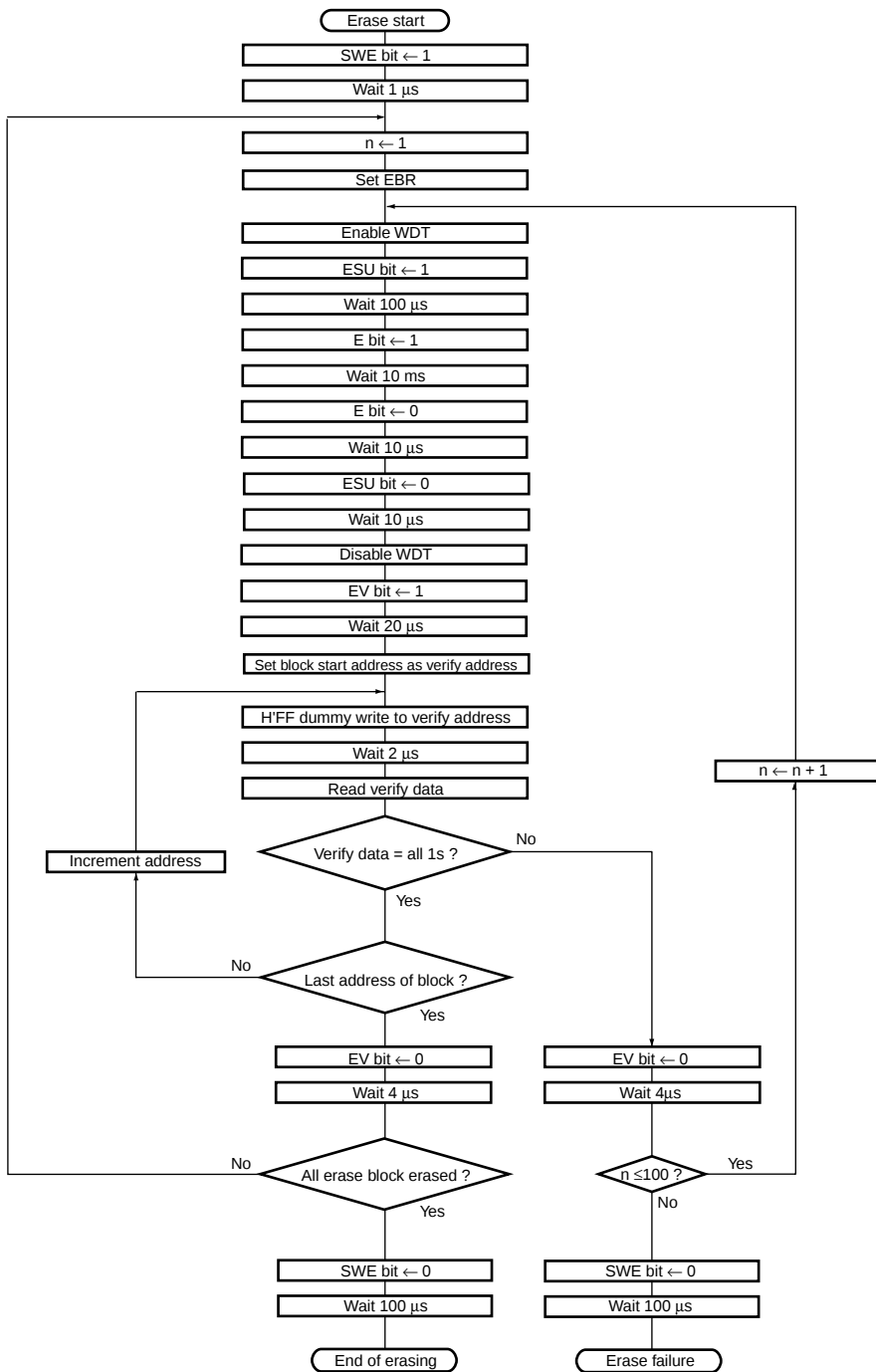
Figure 6.11 Erase/Eraser-Verify Flowchart
