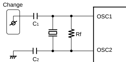
(2) Proposed Change in Oscillator Circuit 1
