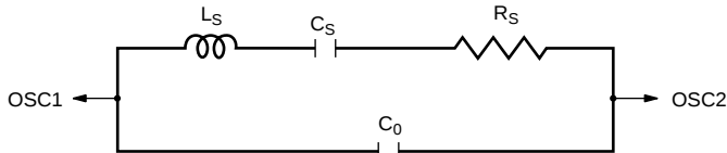
Figure 4.5 Equivalent Circuit of Crystal Resonator
