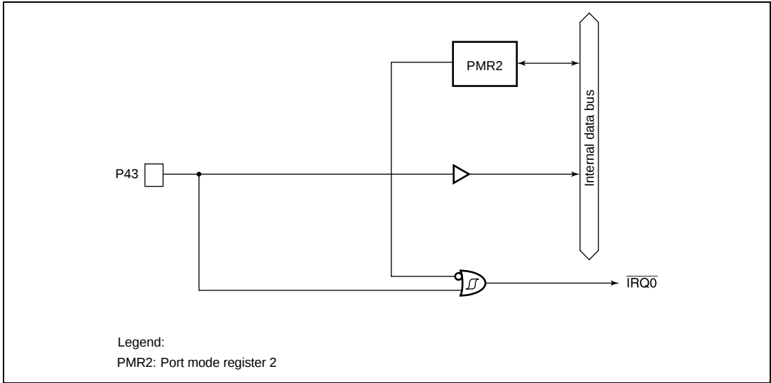
Figure B.2(a) Port 4 Block Diagram (Pin P43)
