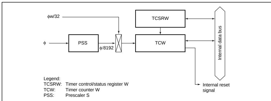
Figure 9.12(1) Block Diagram of Watchdog Timer (H8/38004 Group)
