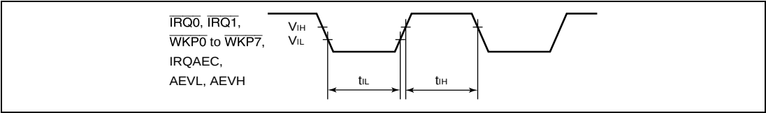
Figure 17.3 Input Timing
