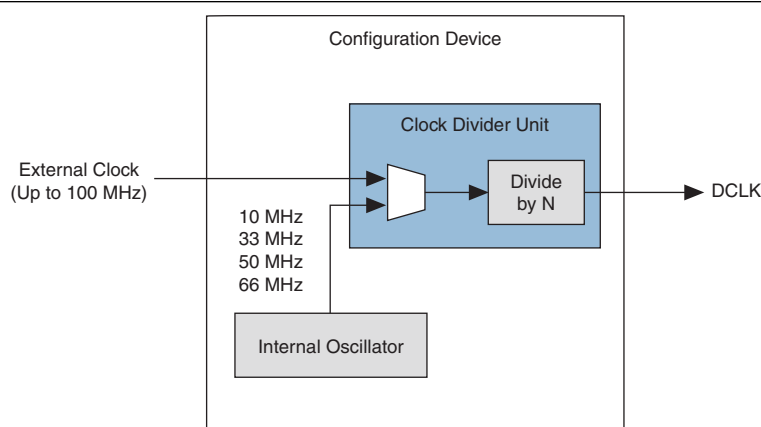
Figure 5. Clock Divider Unit
