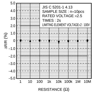
Fig.7 Overload
