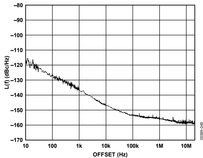
Figure 16. Additive Phase Noise—LVDS DIV2, 122.88 MHz
