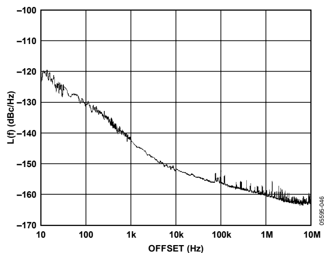
Figure 17. Additive Phase Noise—CMOS DIV4, 61.44 MHz
