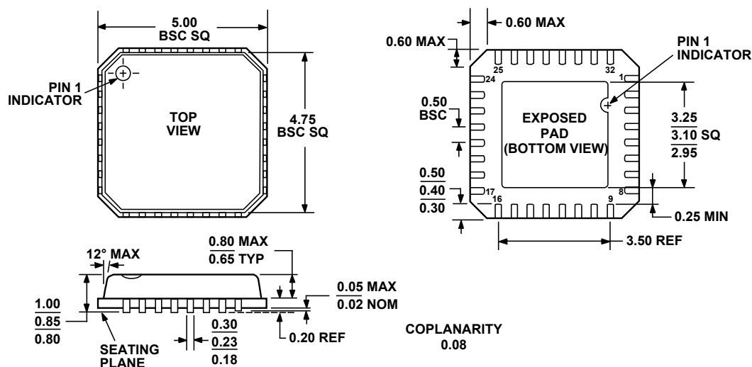
COMPLIANT TO JEDEC STANDARDS MO-220-VHHD-2 Figure 35. 32-Lead Lead Frame Chip Scale Package [LFCSP_VQ] 5 mm x 5 mm Body, Very Thin Quad (CP-32-2) Dimensions shown in millimeters
