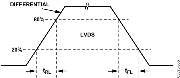
Figure 3. LVDS Timing, Differential
