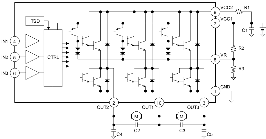
Fig.11 BA6238A
