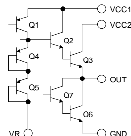
Fig.13 BA6247FP-Y
