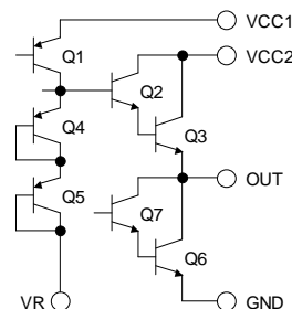
Fig.14 BA6238A
