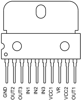
Fig.12 BA6238A (HSIP10)
