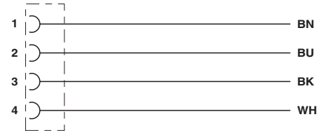
Contact assignment of the DEUTSCH DT06-4S
