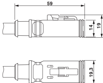
DEUTSCH DT06-4S, top view and side view
