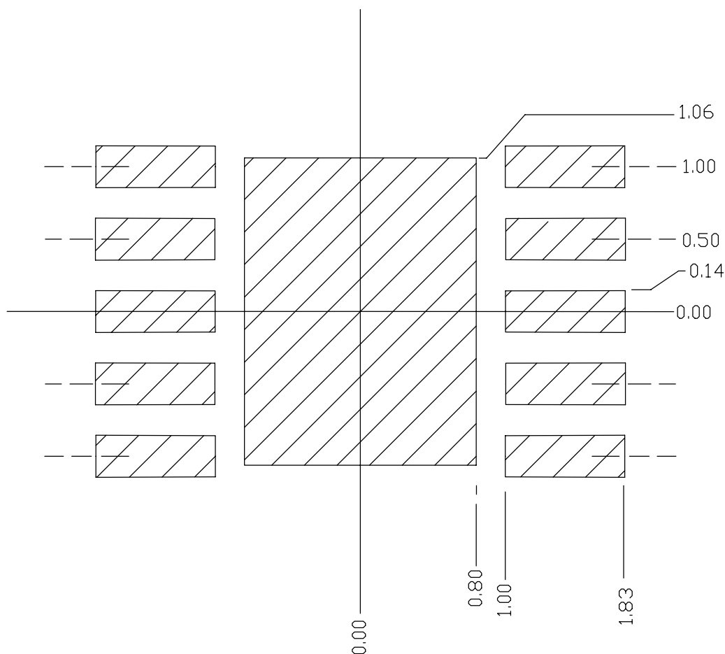
SUGGESTED PCB LAND PATTERN
