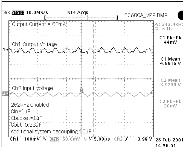
Ripple Voltage
