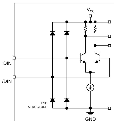
Figure 2. Input Structure
