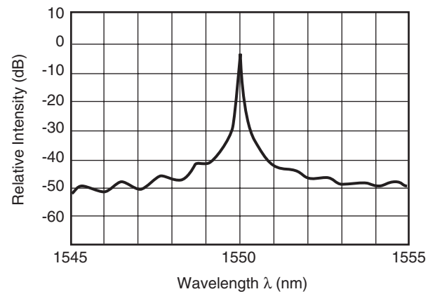
Fig.4 Spectrum
