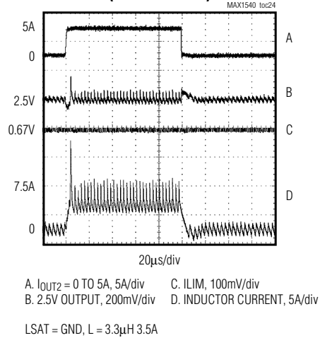
INDUCTOR-SATURATION PROTECTION (LSAT DISABLED)
