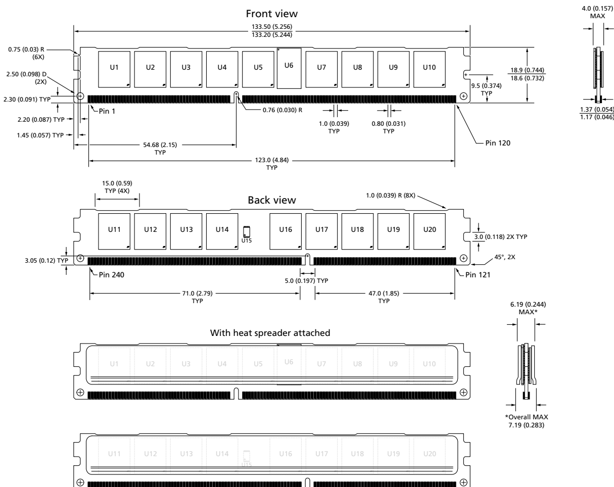
Figure 3: 240-Pin DDR3 RDIMM
