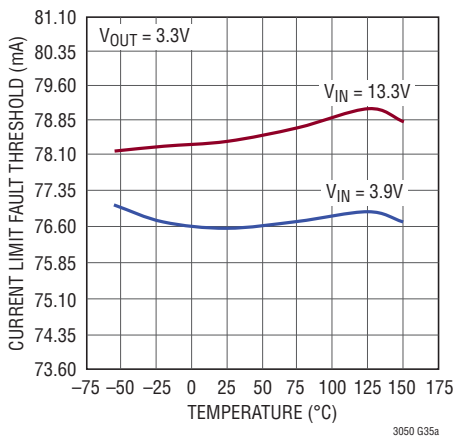
External Current Limit R_{IMAX} = 1.5k
