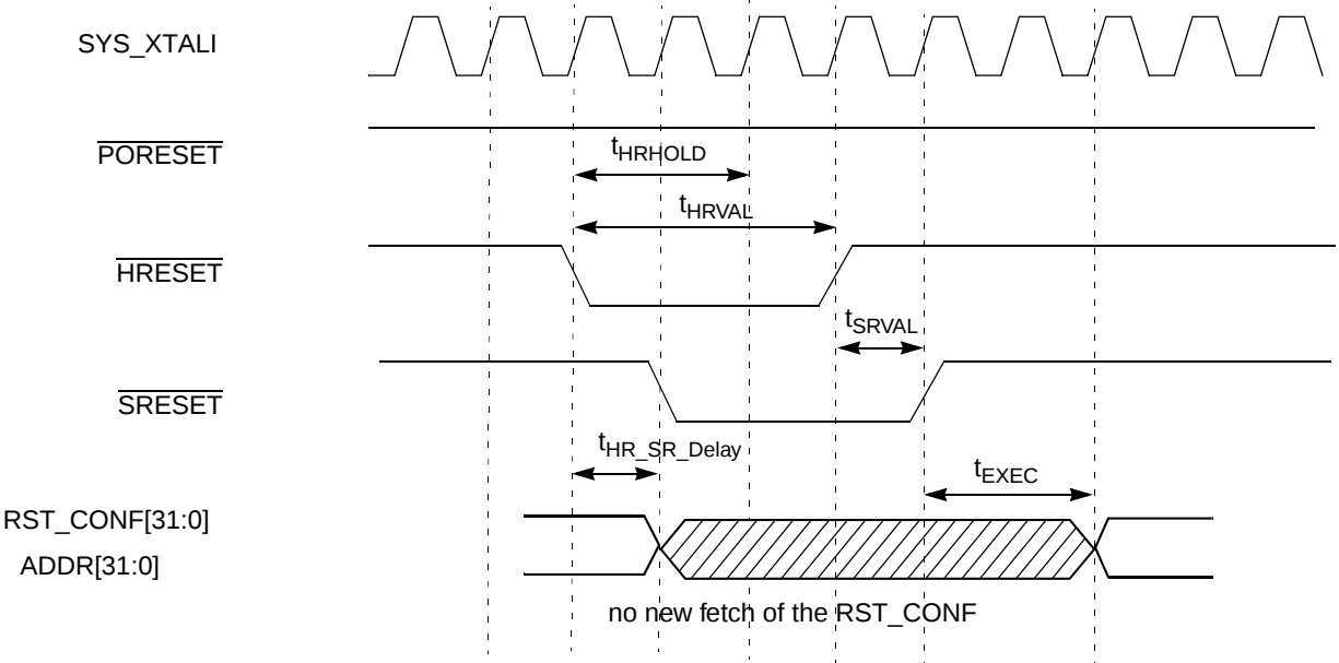
Figure 6. HRESET Behavior
