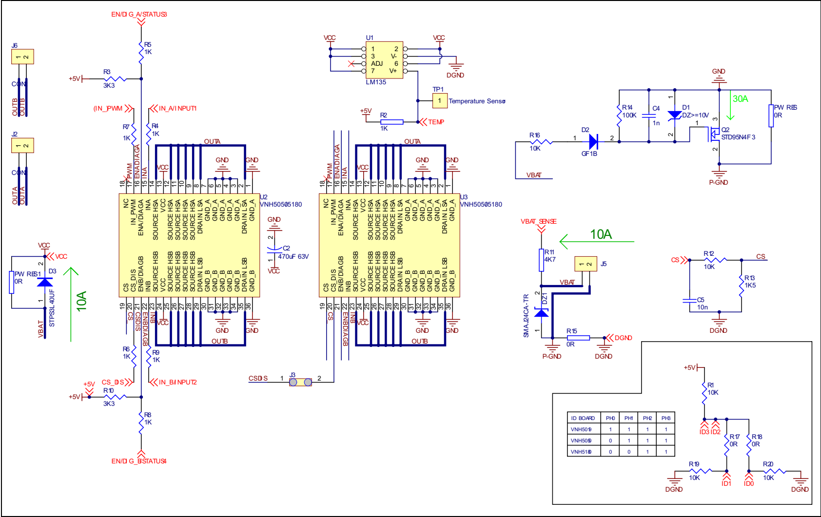
Figure 4. VNH5180A daughterboard application schematic (part 2)
