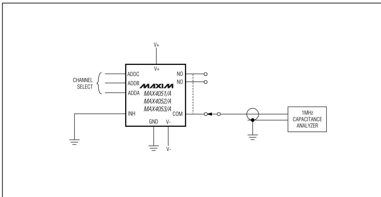
Figure 7. NO/COM Capacitance
