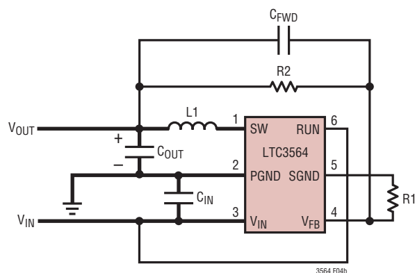
Figure 4b. LTC3564 DFN Layout Diagram
