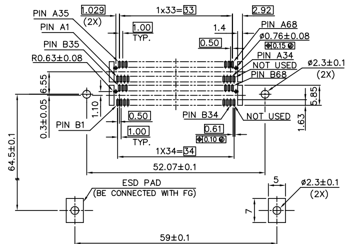
RECOMMENDED P.C.B. LAYOUT 2 (MOUNTED SIDE)
