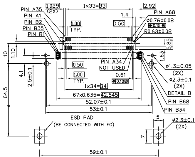
RECOMMENDED P.C.B. LAYOUT 1 (MOUNTED SIDE)
