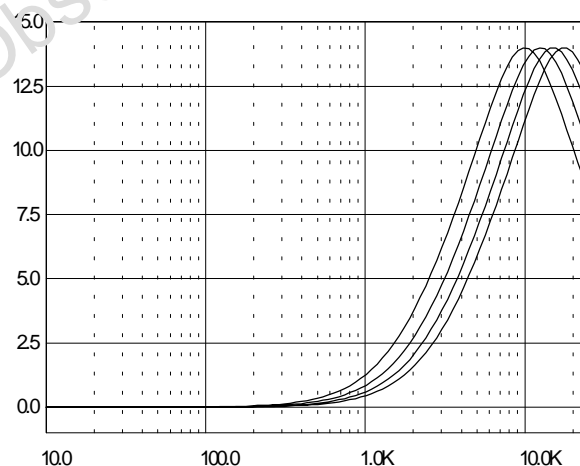
Figure 11. Treble Center Frequencies @ Gain = 14dB
