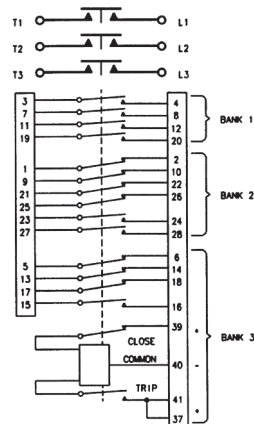
Circuit Configuration 1
