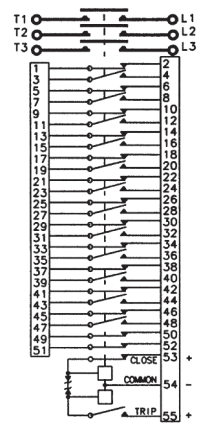
Circuit Configuration 2
