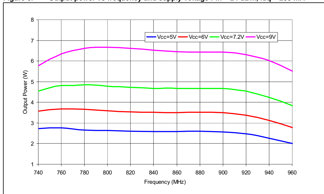
Figure 6. Output power vs frequency and supply voltage P_{in} = 24\text{ dBm} , I_{dq} = 200\text{ mA}
