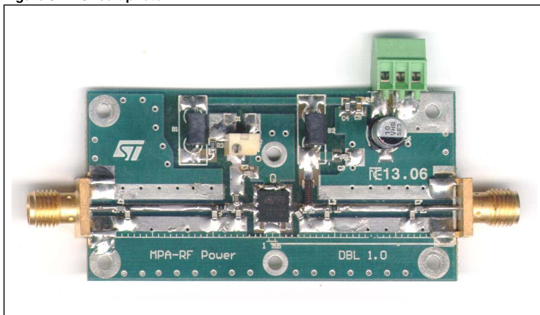
Figure 8. Circuit photo
