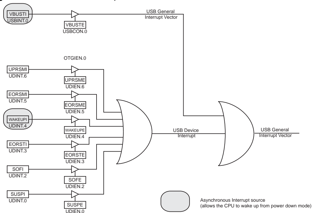
Figure 21-9. USB General interrupt vector sources
