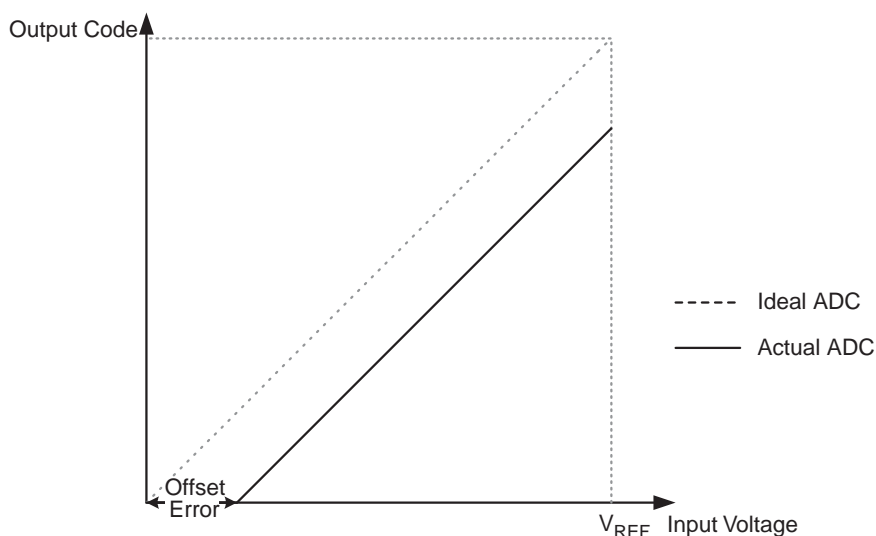
Figure 24-11. Offset Error
