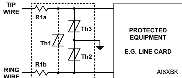
Figure 17. Protection Module
