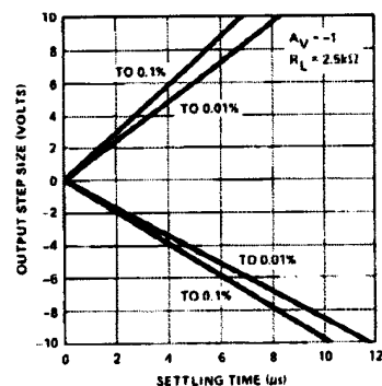
SETTLING TIME
