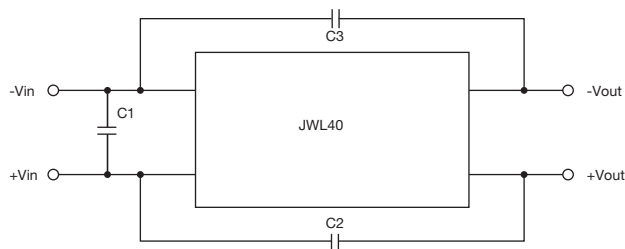
Single Output
