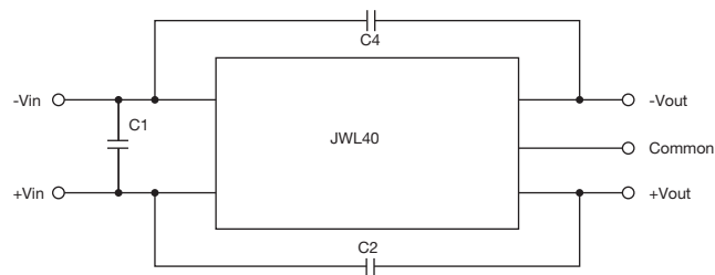
Dual Output
