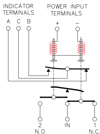
Indicators
