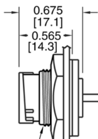
CABLE END CONNECTOR STYLE 5 LONG TWIST LOCK BACKSHELL
