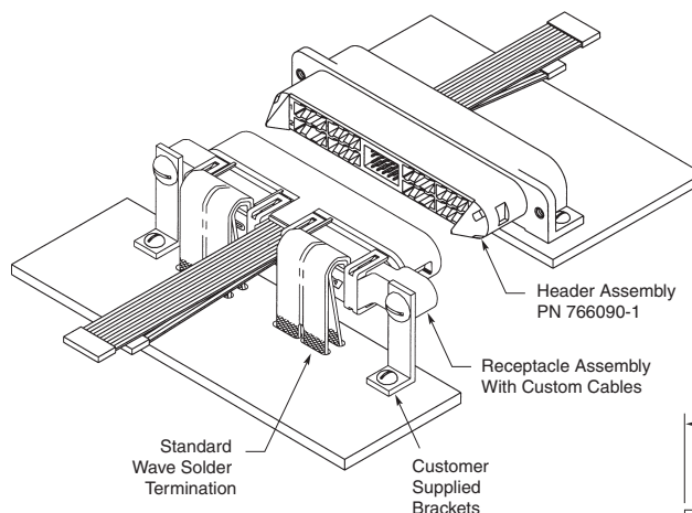
Floating Receptacle
