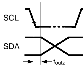
Figure 29. Data Output Timing
