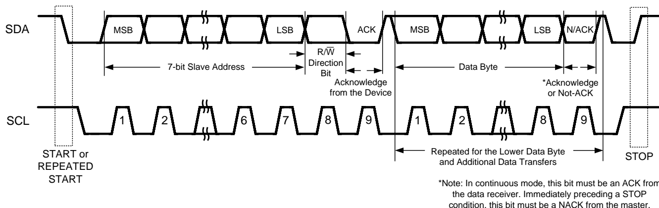
Figure 24. Basic Operation.
