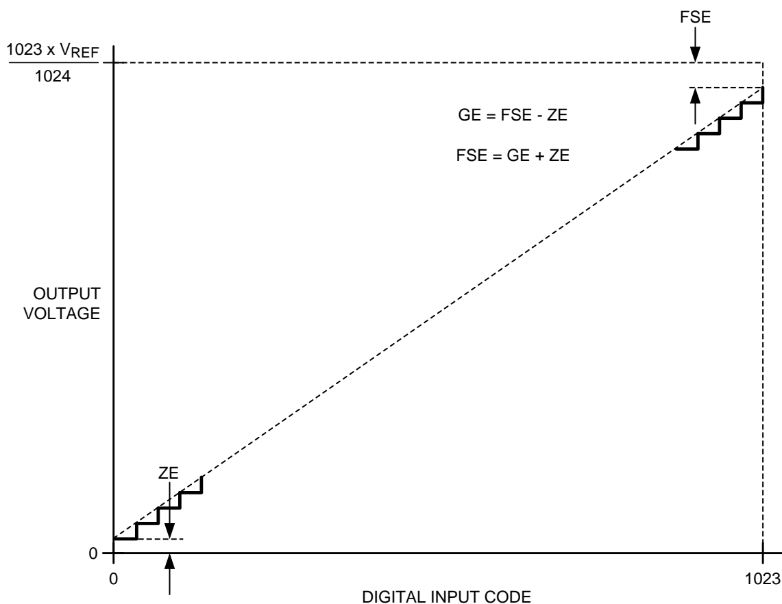
Figure 4. Input / Output Transfer Characteristic
