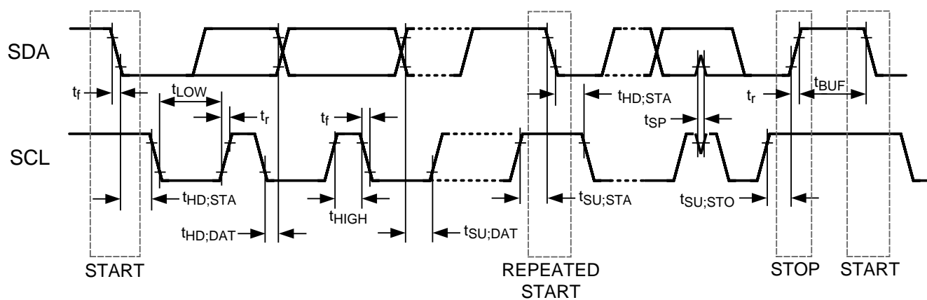
Figure 5. Serial Timing Diagram
