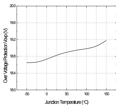
Figure 12. Over Voltage Protection Level
