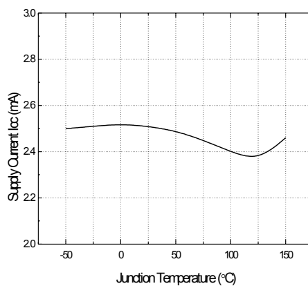
Figure 2. Supply Current
