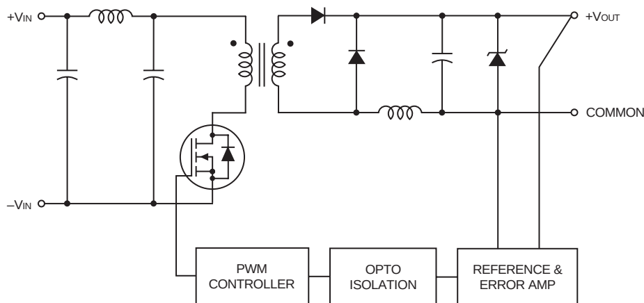
Figure 1. Simplified Schematic
