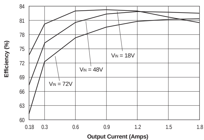
Efficiency vs. Output Current and Input Voltage
