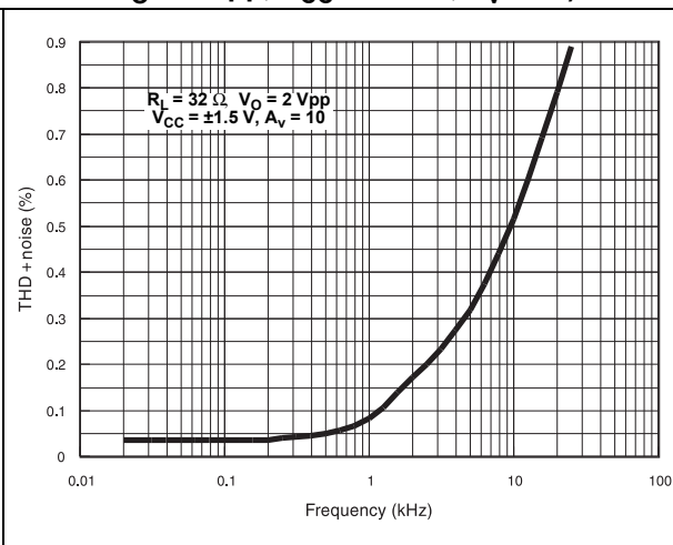
Figure 8. THD + noise vs. frequency ( R_L = 32\ \Omega , V_O = 2\text{ Vpp} , V_{CC} = \pm 1.5\text{ V} , A_V = 10 )
