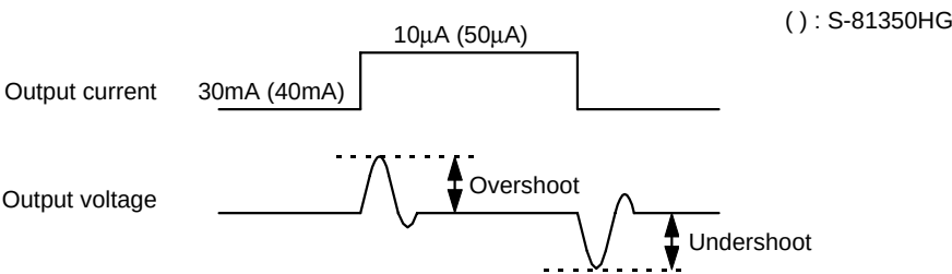
Figure 12 Ringing waveform
