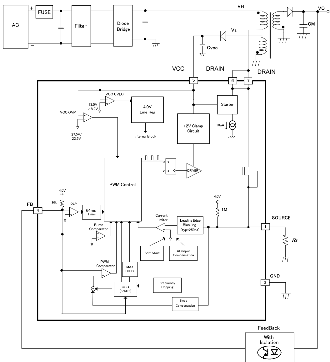
Figure 3. Block Diagram
