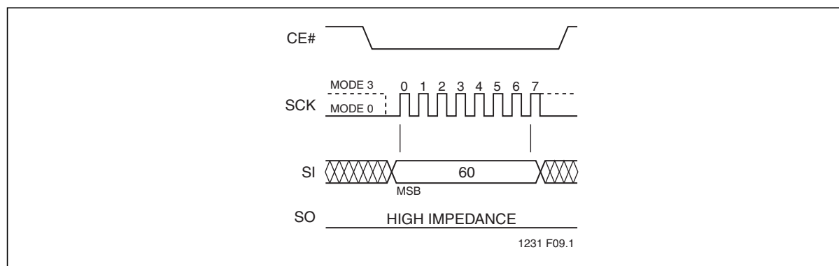
Figure 10: Chip-Erase Sequence
